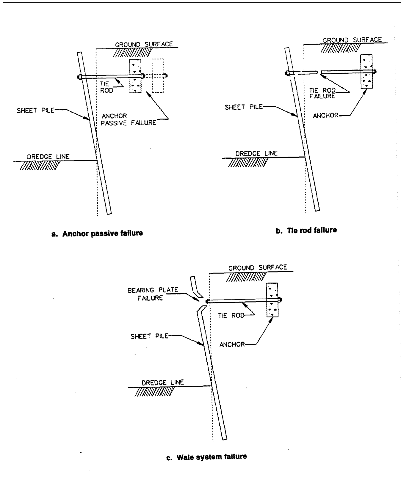
Figure 5-4. Anchorage failures
